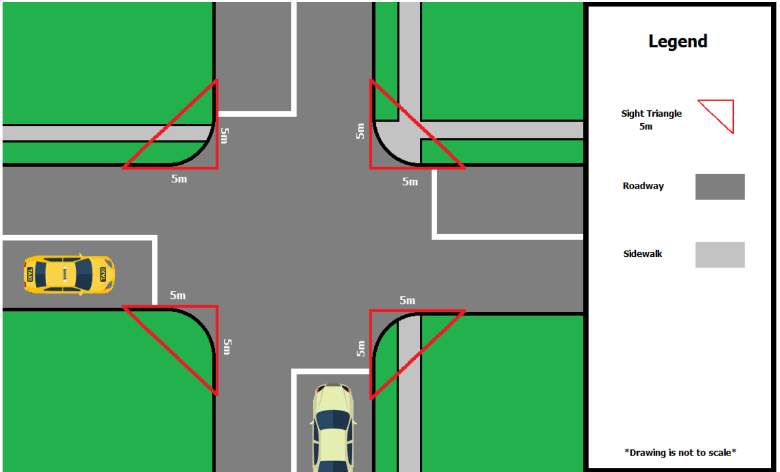
Diagram 1 – Sight triangle
